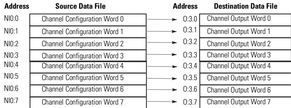
Figure 5.3 Copy File Data Flow
