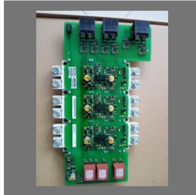
Thyristor / IGBT / Driver Board /Semiconductor
