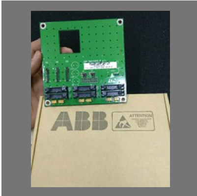
ABB Gate Driver Trigger Board, CODE- 68242843 TYPE- AGBB-01C
