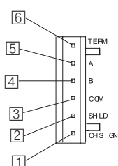
DH-485 connector Port 3
